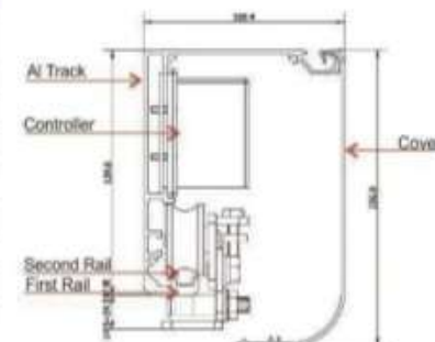
Cross Section of Aluminum Track
