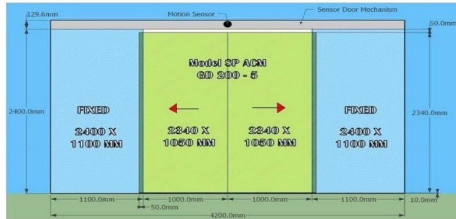
Picture – 1 (Door Layout – front View)
